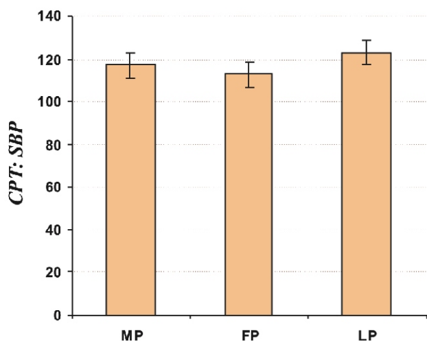
Graph 5: Comparison of SBP response to cold pressor test (CPT) between the phases-MP,FP and LP.
